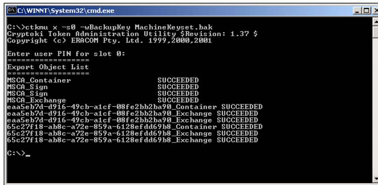
Figure 3 - Backup Keyset
