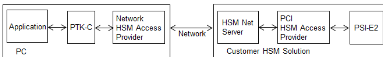
Figure 3: Network Mode using a SafeNet ProtectServer adapter
