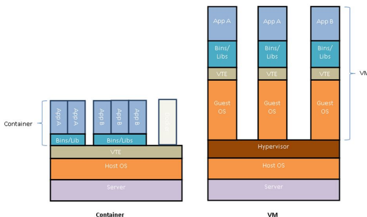
Figure 12-1: CTE in Docker container environment versus virtual machine environment
