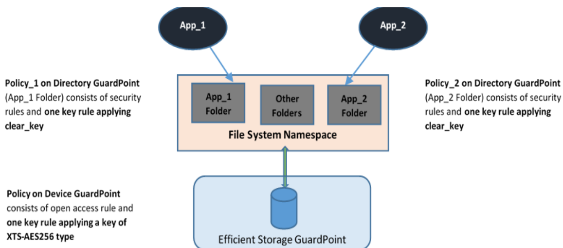
Figure 13-2: All Data in file system Device Encrypted through an ES GuardPoint
